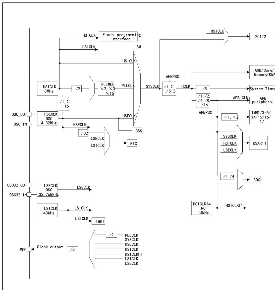
Figure 3 Clock tree of APM32F030x6x8
